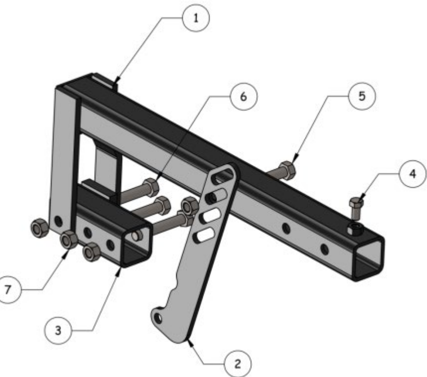
Left Mount Arm, Early Models (Direct Drive Reel)
