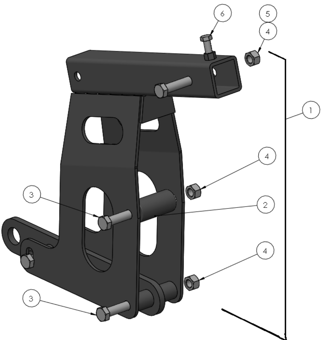
Outer Mount Arm (Right Hand)
