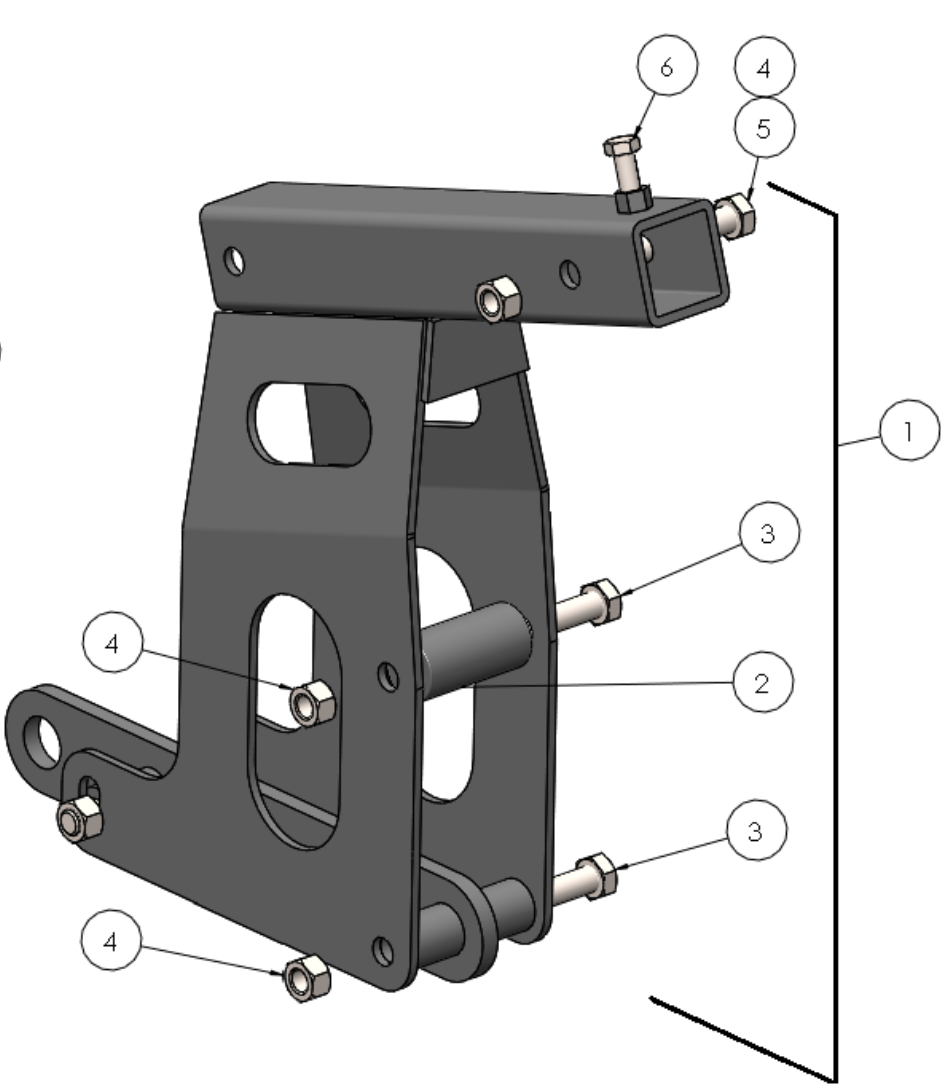
Outer Mount Arm (Left Hand)
