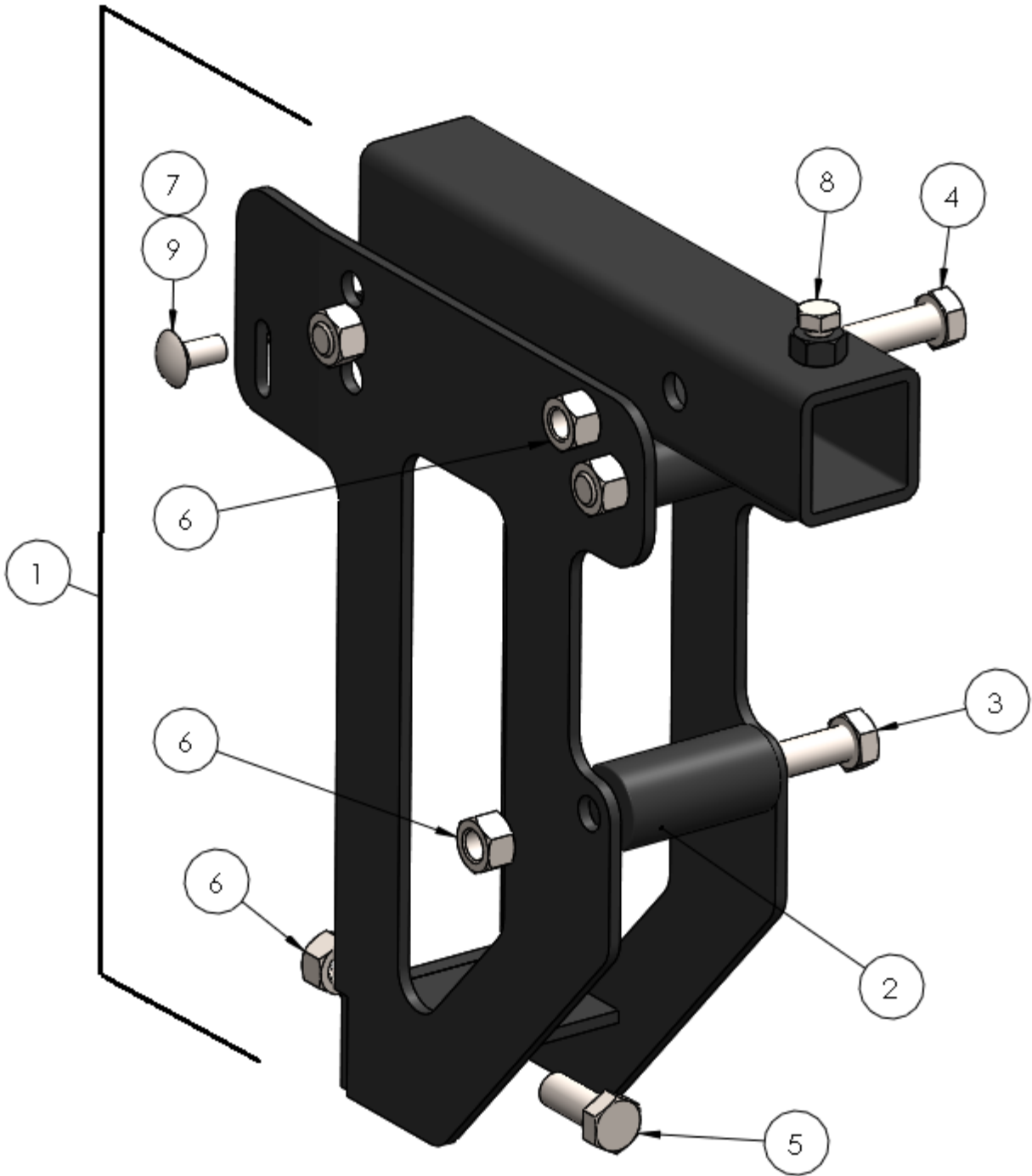
FD70 Mount Arm Bracket (Left Hand and Center)
