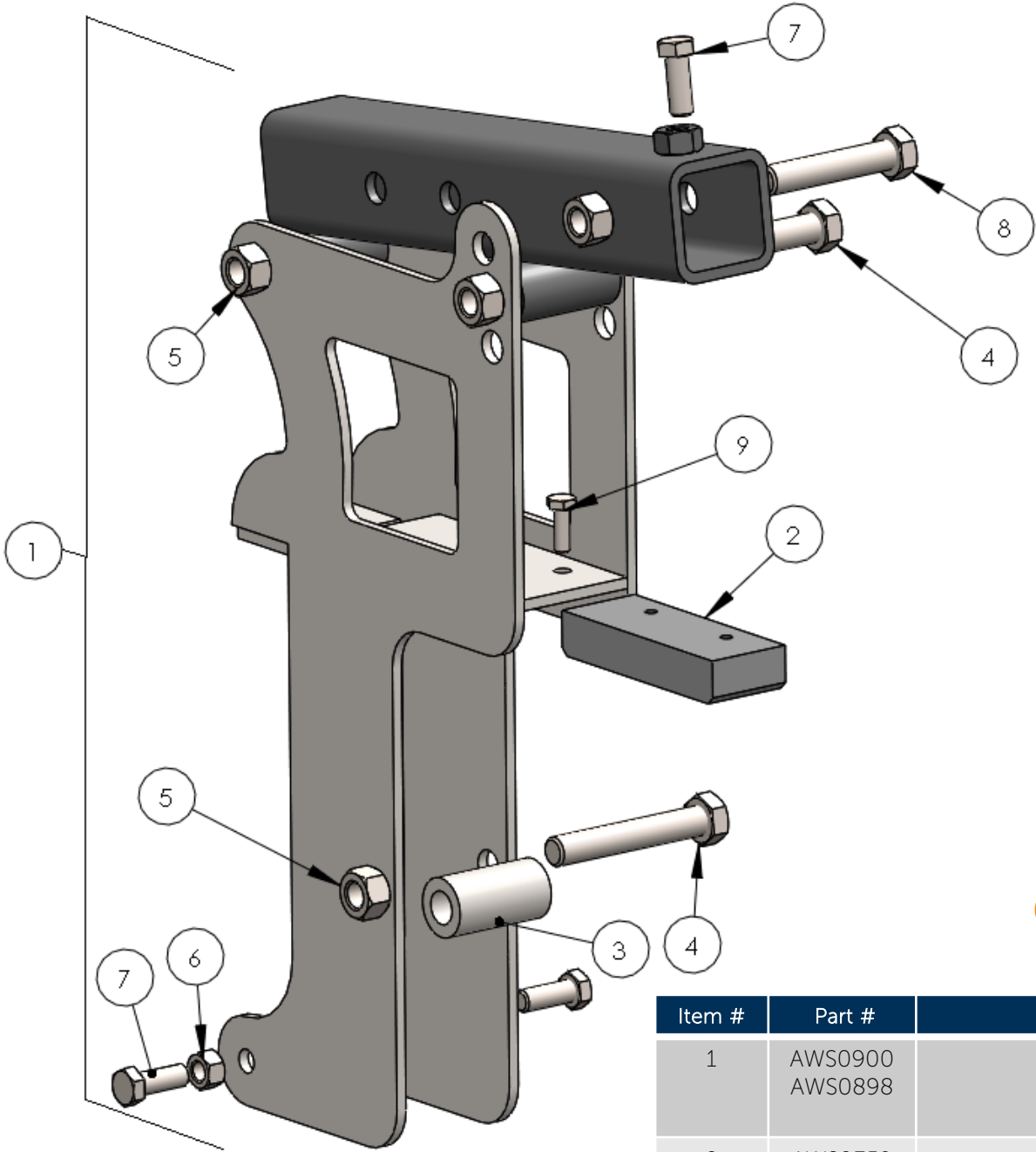
Outer Brackets (LH Shown)
