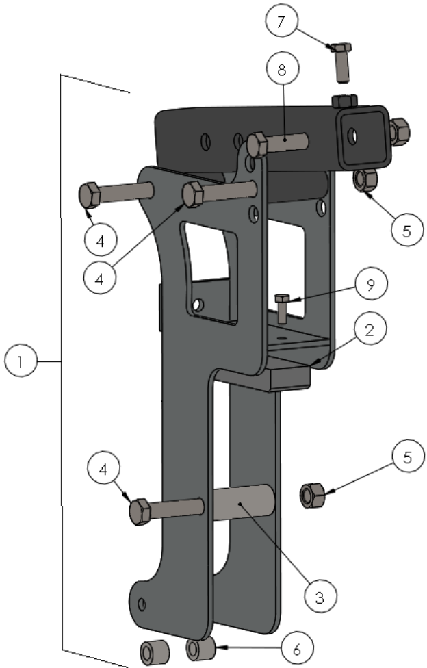
JD 30-35ft Mount Arm, Right
