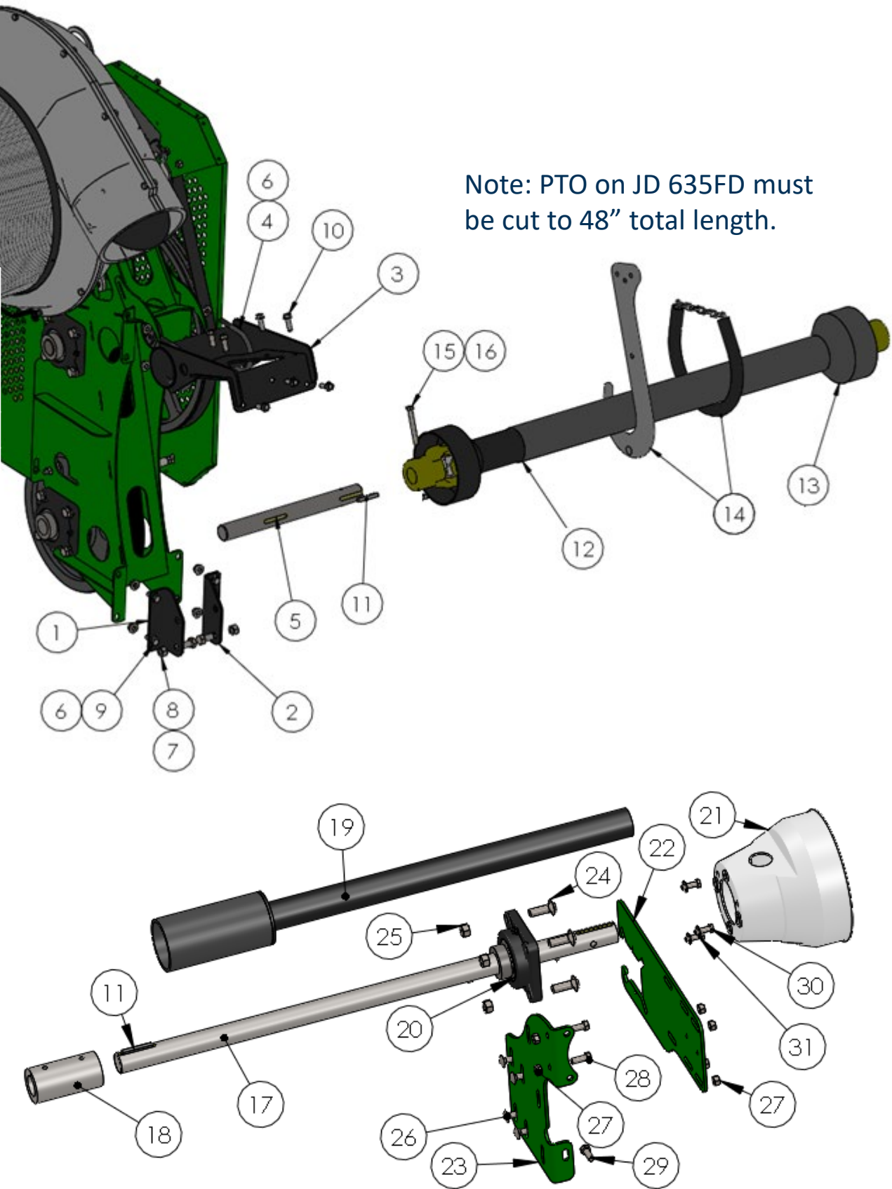
Driveline Extension For 45'
