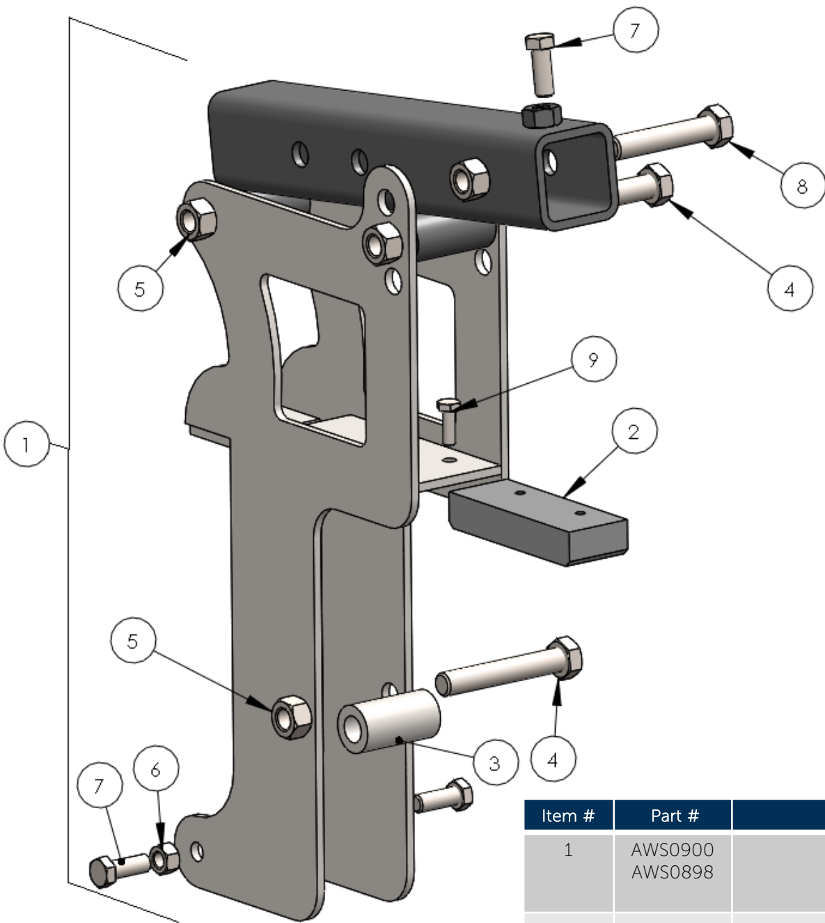
Outer Brackets (LH Shown)
