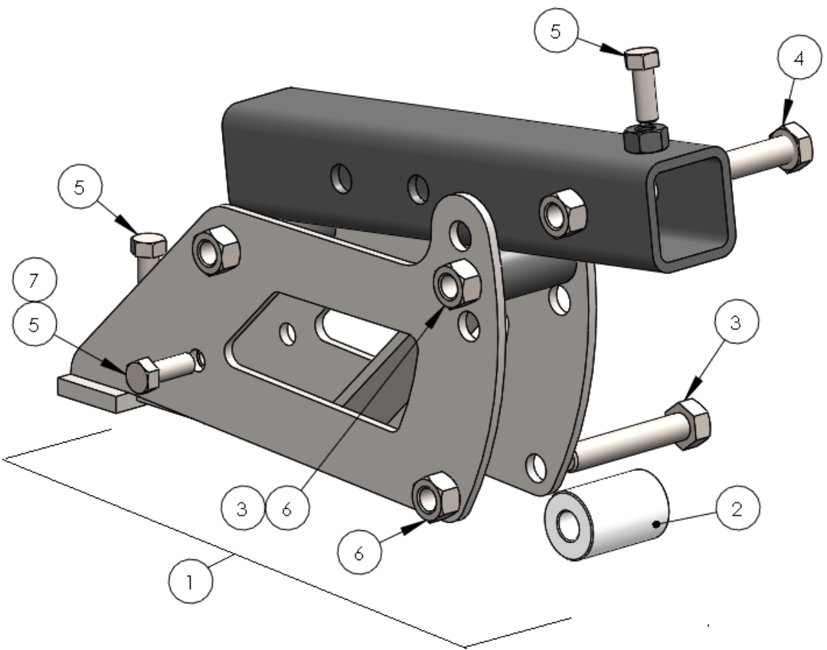
Centre Bracket
