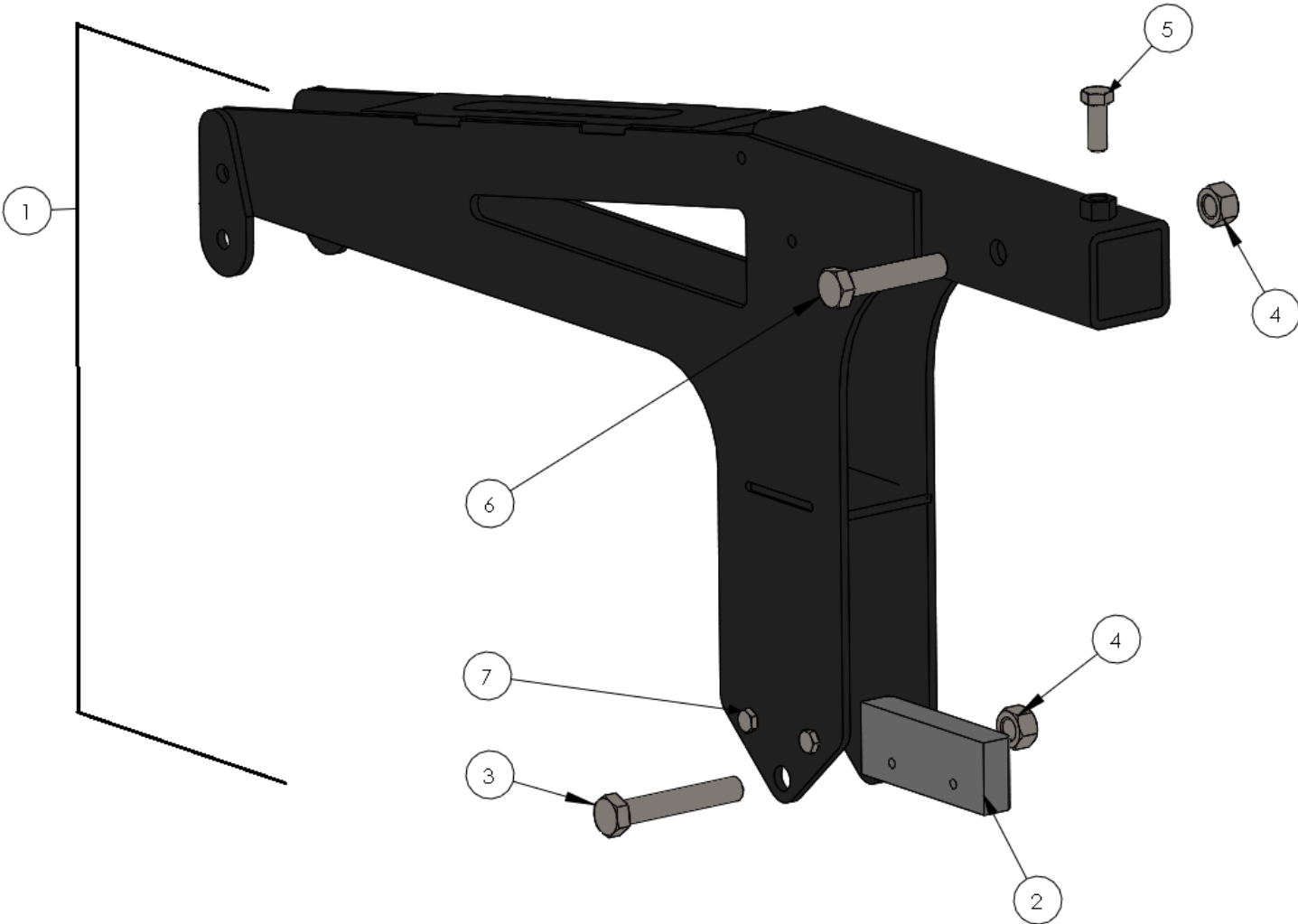
Centre Mount Arm Assy.
