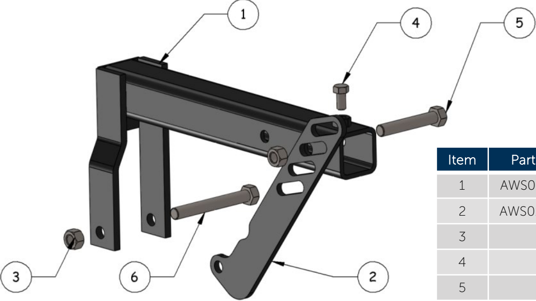
Left Assembly, Hart-Carter Reel
