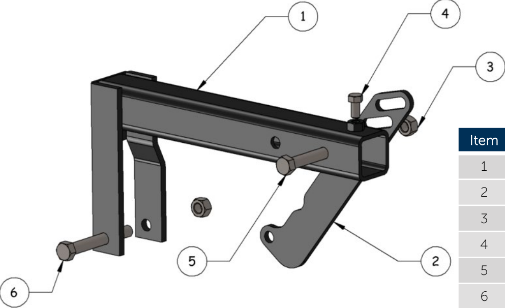
Right Assembly, Hart-Carter Reel
