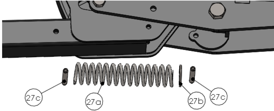
Cushioned Manifold 2018-
