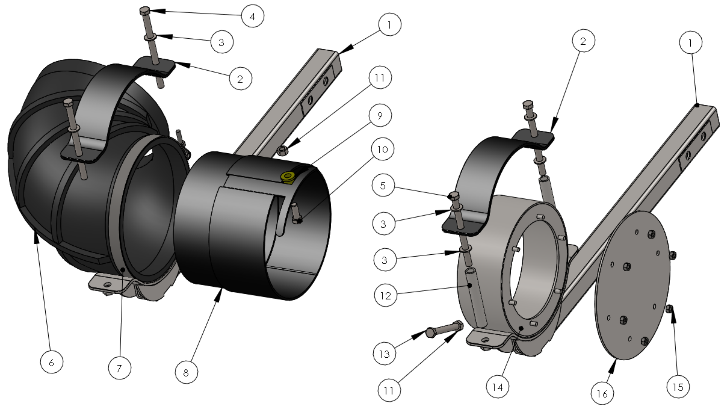
AWS0819 End Cap Assembly, w/o Lever, includes items 11,13,14,15,16 and replaces AWS0616 End Cap, no lever(-2015)
