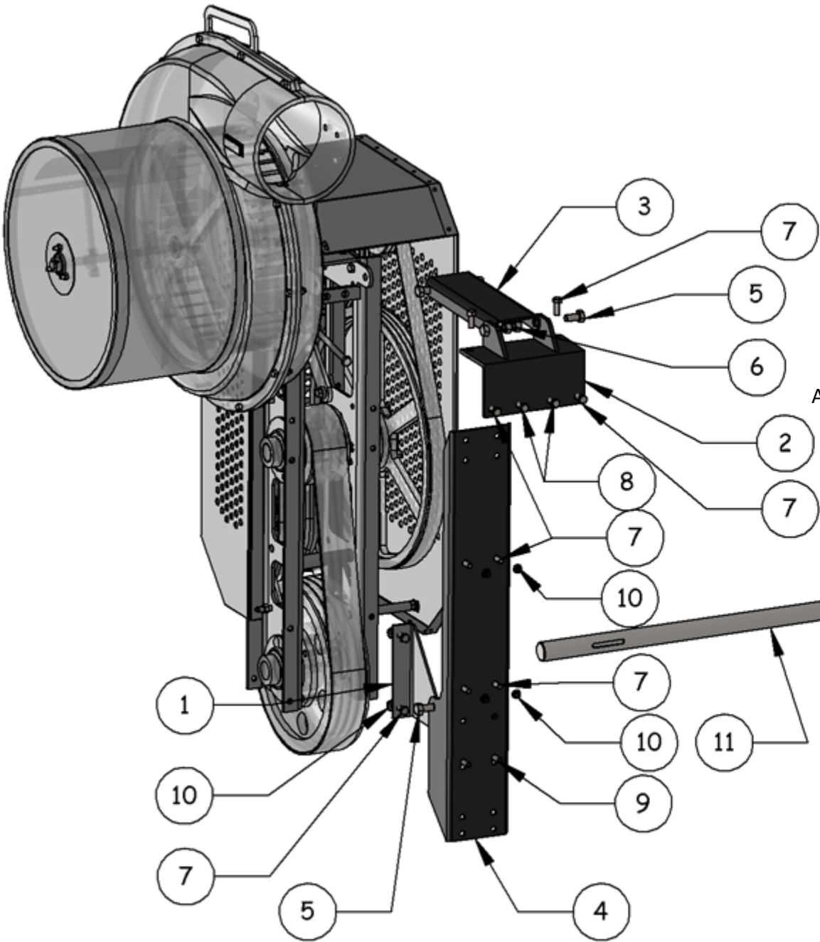
View A: Bearing Support Assembly (JD 630 and 635 Headers Only)
