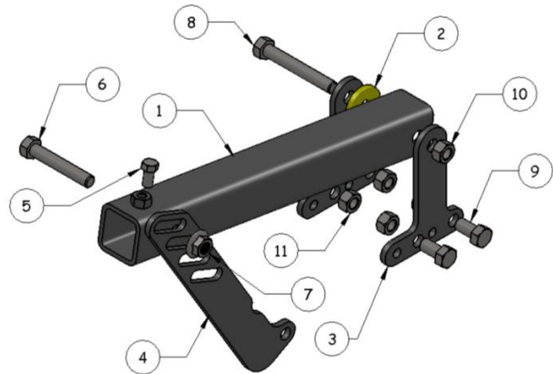
Right Mount Arm Assy. AWS0244
