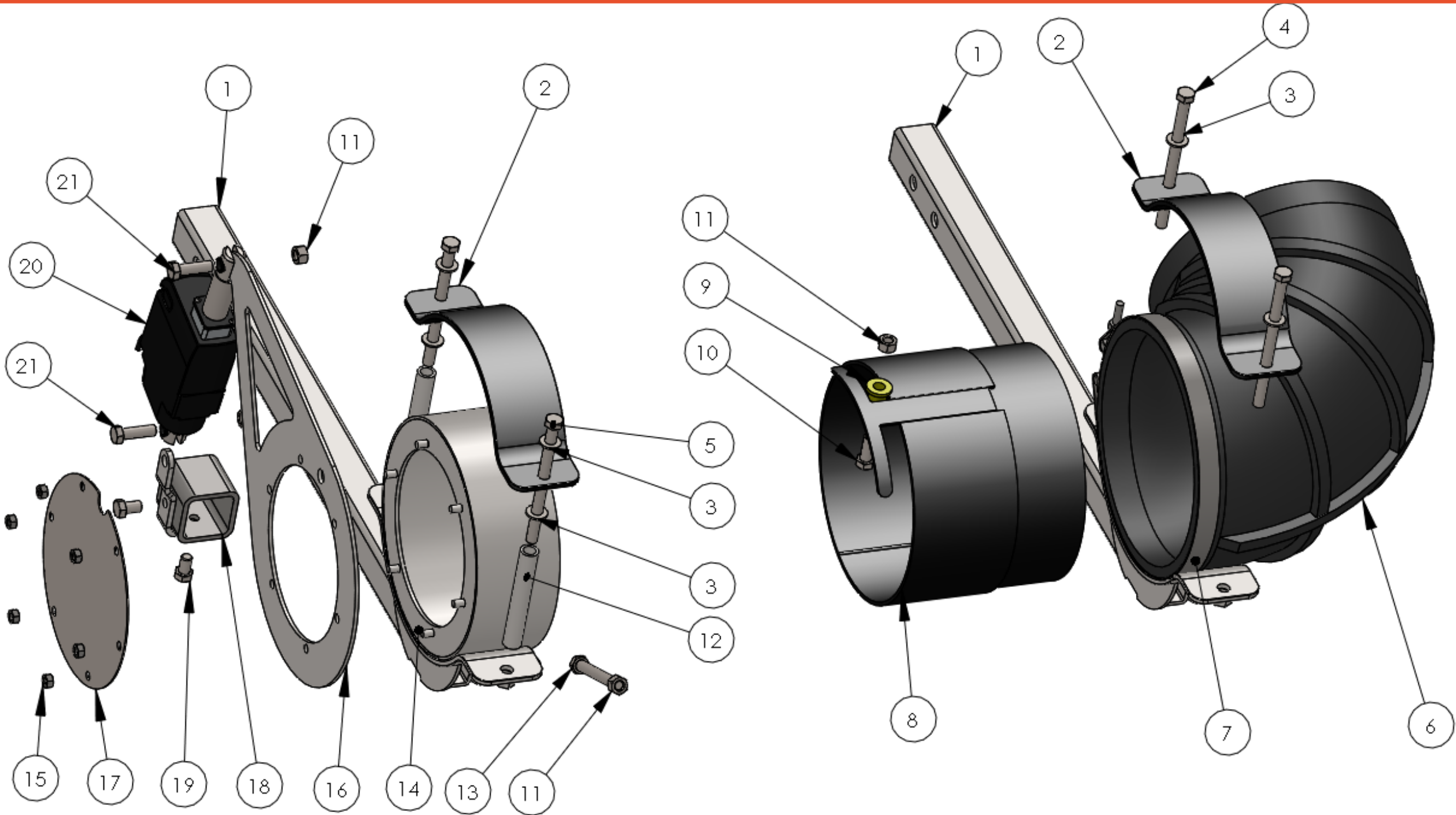
AWS0814 End Cap Assembly, w/ lever includes items 11,13,14,15,16,17 and replaces AWS0094 End Cap (-2015)
